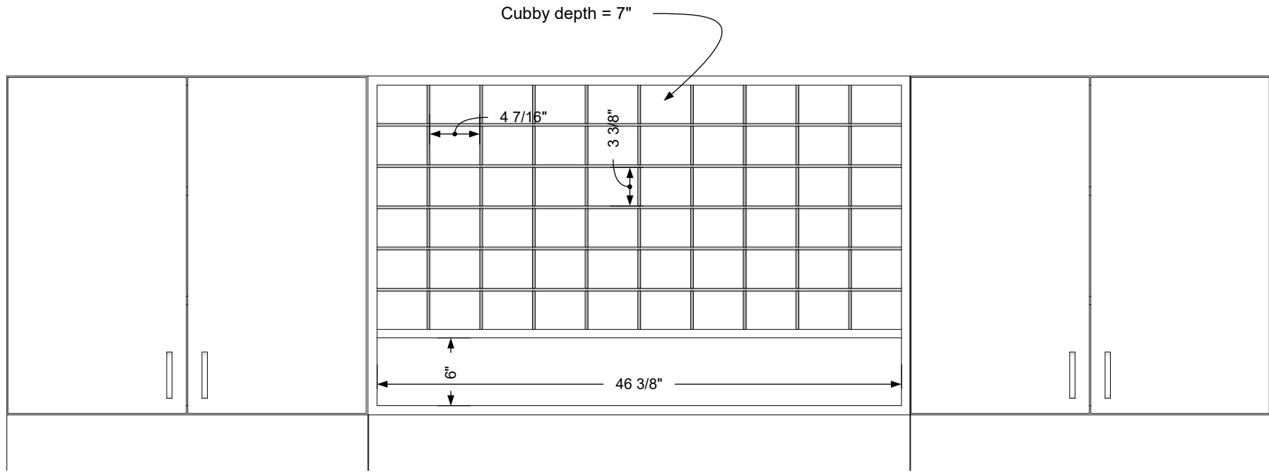
Cubby details
