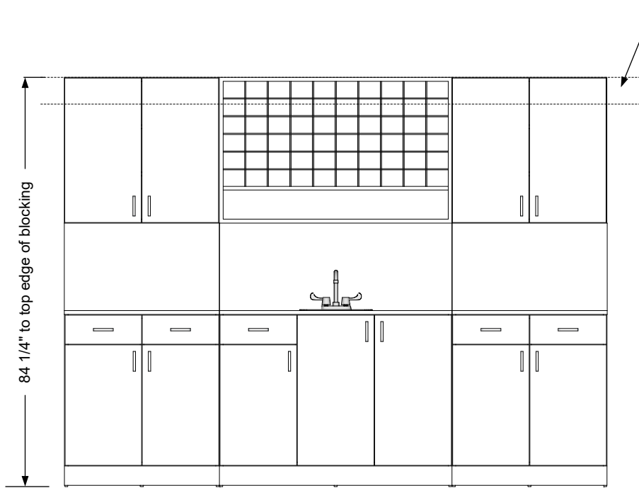
Blocking detail
