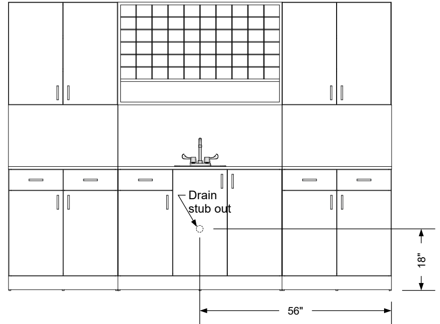
Plumbing stub out detail
