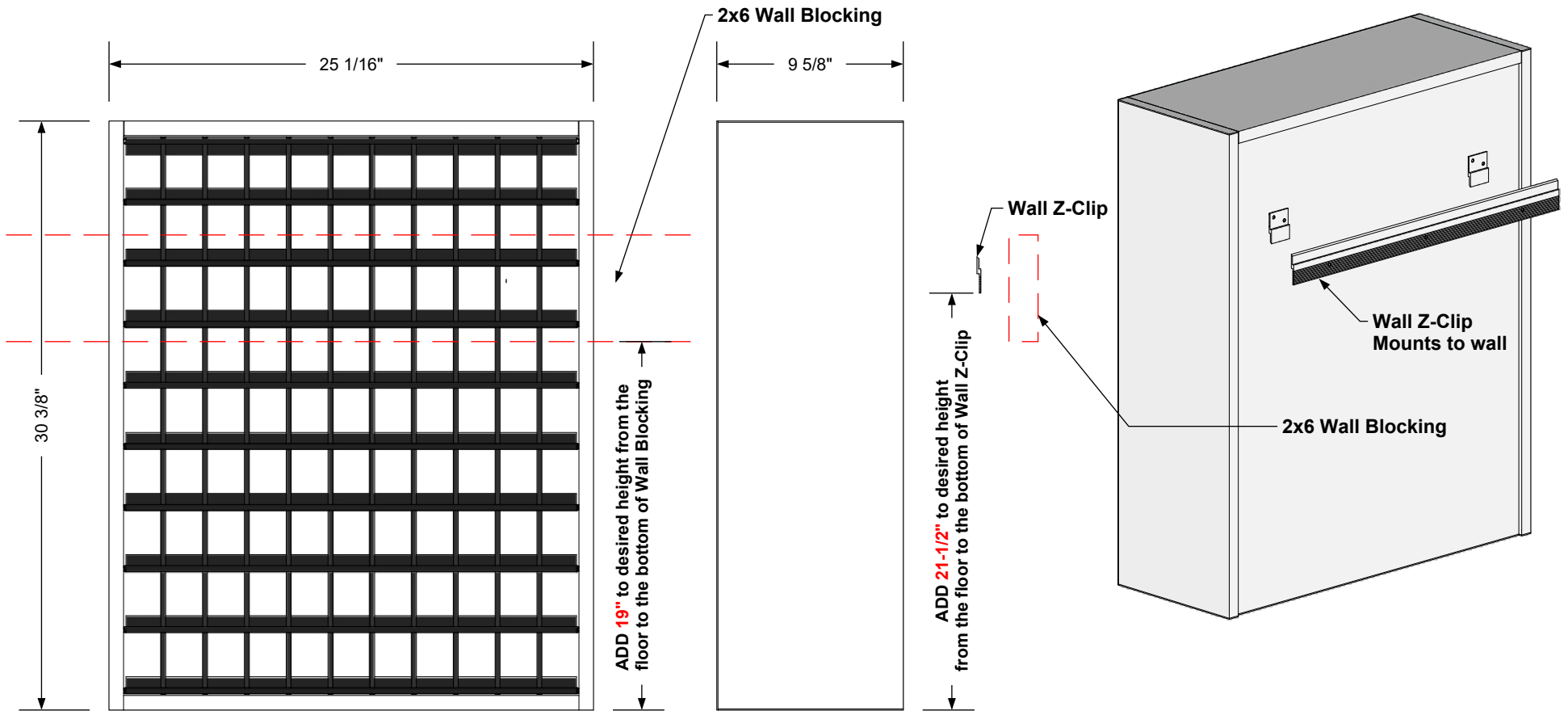
Typical Starting Height Of Cabinet 54" After Finished Floor.
